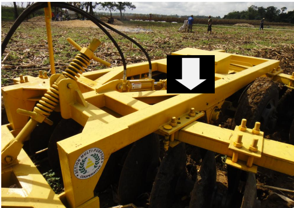
Figure 6. Main frame
