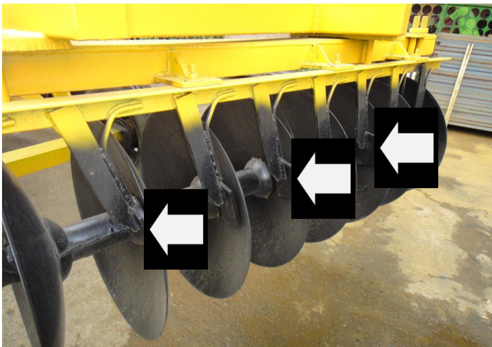
Figure 3. Scrapers
